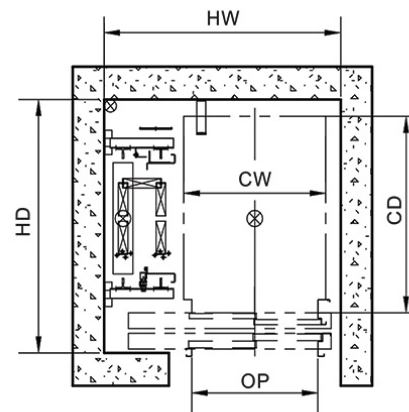
Hoistway Plan
